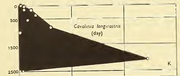
TEXT-FIG. 1.—Vertical distribution by day and night of the more abundant species: A, B, Creseis acicula ; C, D, Hyalacylis striata ; E, F, Clia pyramidata ; G, H, Diacria quadridentata ; J, K, Cavalinia longirostris .
